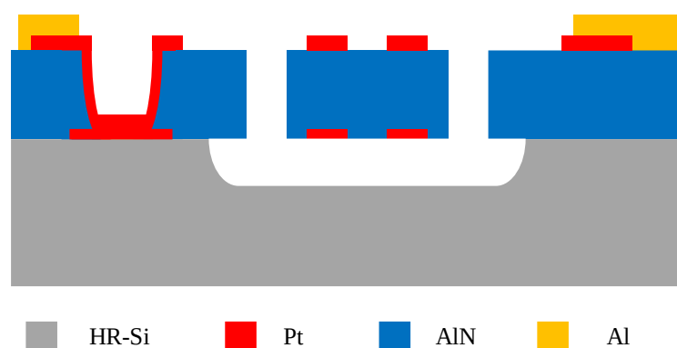
Figure 1 Process Cross-Sectional View
